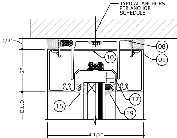
1.1 HEAD DETAIL WET GLAZE
