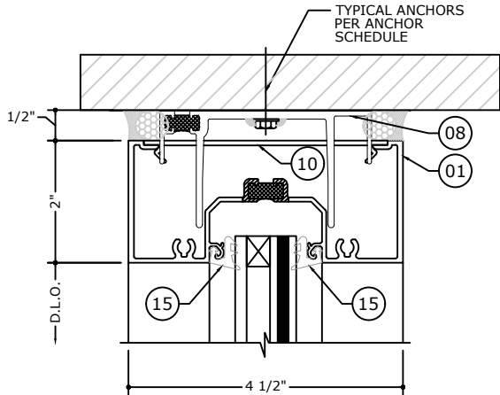
1 HEAD DETAIL DRY GLAZE
