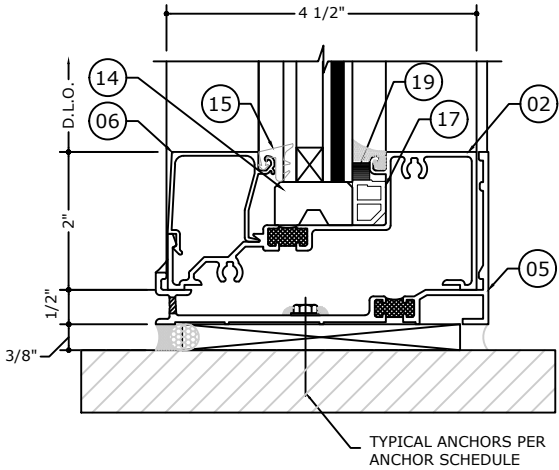
3.1 SILL DETAIL WET GLAZE
