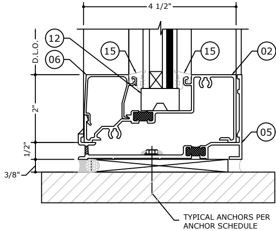
3 SILL DETAIL DRY GLAZE
